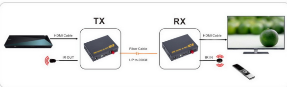
DD474 HDMI Fiber Optic Extender Support Max Resolution 1080P@60Hz Transmission distance: standard 20km (compression); maximum 80km, Black, Metal case
